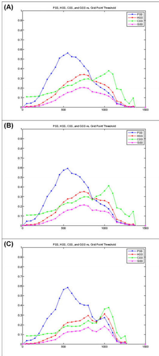
Figure 10: a) Same as Fig. 6d. b) As in (a), for 630 training cases. c) As in (a), for 420 training cases. Click image to enlarge.
