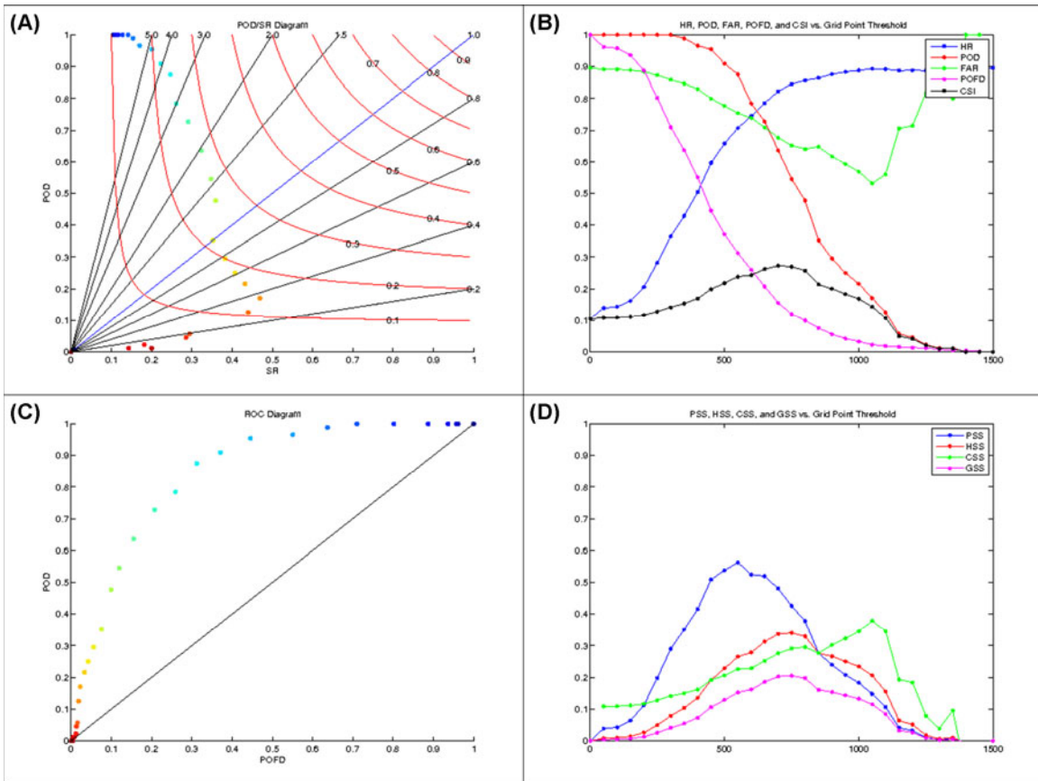
Figure 6: As in Fig. 5, with outbreak classification modified by using the N15 index rather than the N25 index. Click image to enlarge.
