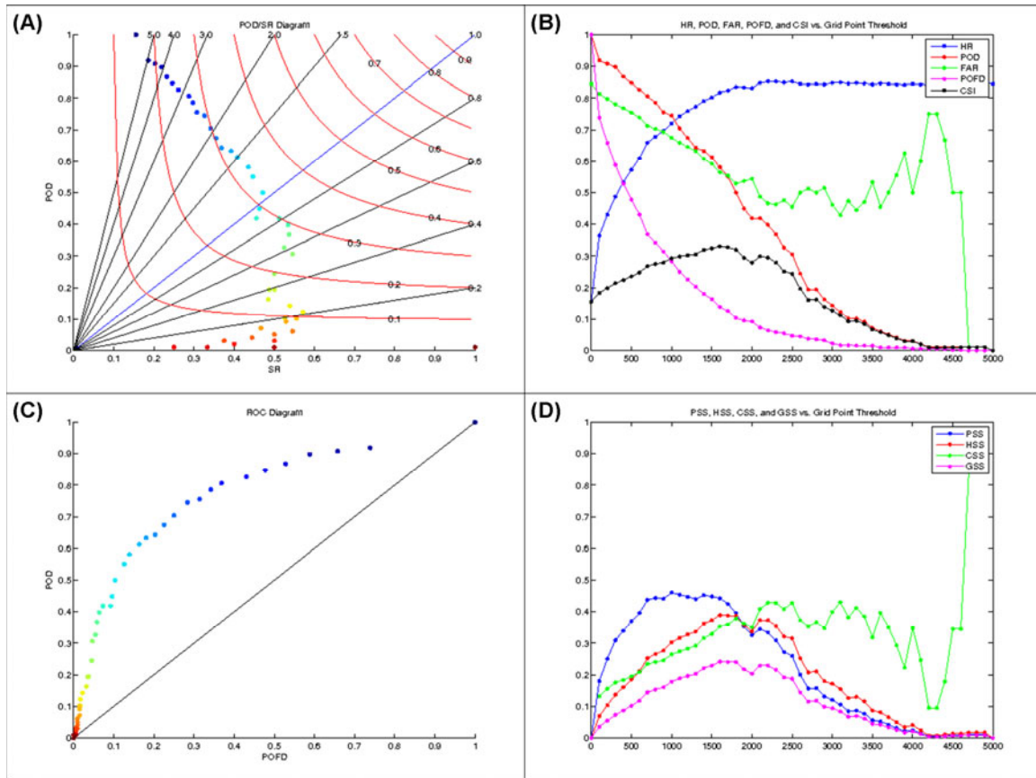
Figure 8: As in Fig. 4, for the training cases only. Click image to enlarge.
