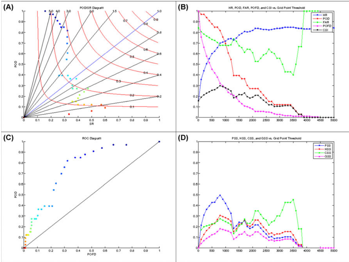
Figure 9: As in Fig. 4, for the testing cases only. Click image to enlarge.
