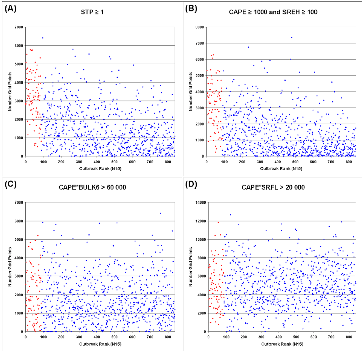
Figure 2: Number of grid points exceeding a) a threshold value of 1 for STP, b) a threshold value of 1000 \text{ J kg}^{-1} SBCAPE and a threshold value of 100 \text{ m}^2 \text{ s}^{-2} for 0–1 km SREH, c) a threshold value of 60 000 for the product of SBCAPE ( \text{J kg}^{-1} ) and 0–6 km bulk shear (kts), and d) a threshold value of 20 000 for the product of SBCAPE ( \text{J kg}^{-1} ) and SRFL ( \text{m s}^{-1} ), for each of the 840 cases. Cases ranked in order from 1 to 840 using the N15 index. Major (intermediate or marginal) outbreaks are indicated by red (blue) dots. Click image to enlarge.
