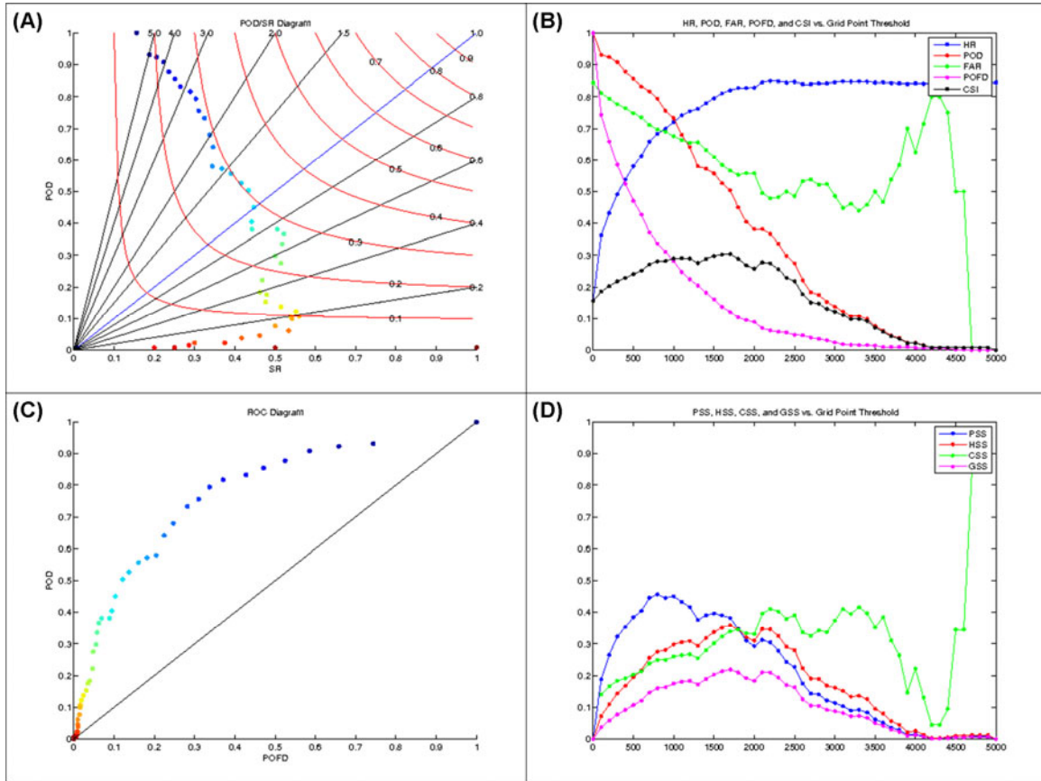
Figure 4: a) Roebber (2009) diagram, using the total number of land grid points for the constrained STP \geq 1 for diagnosis of outbreak type and the N25 index for outbreak classification. Bias is shown using diagonal black lines (with the blue line showing a bias of unity). Red curves indicate CSI. Individual points indicate grid point thresholds in increments of 100, starting from 0 (blue) to 5000 (maroon). b) Hit rate (blue), probability of detection (red), false alarm ratio (green), probability of false detection (magenta), and critical success index (black) of the grid point thresholds specified on the x -axis. c) Relative operating characteristics (ROC) diagram for each of the grid point thresholds, as in (a). d) Pierce (blue), Heidke (red), Clayton (green), and Gilbert (magenta) skill scores for each of the thresholds in (b). Click image to enlarge.
