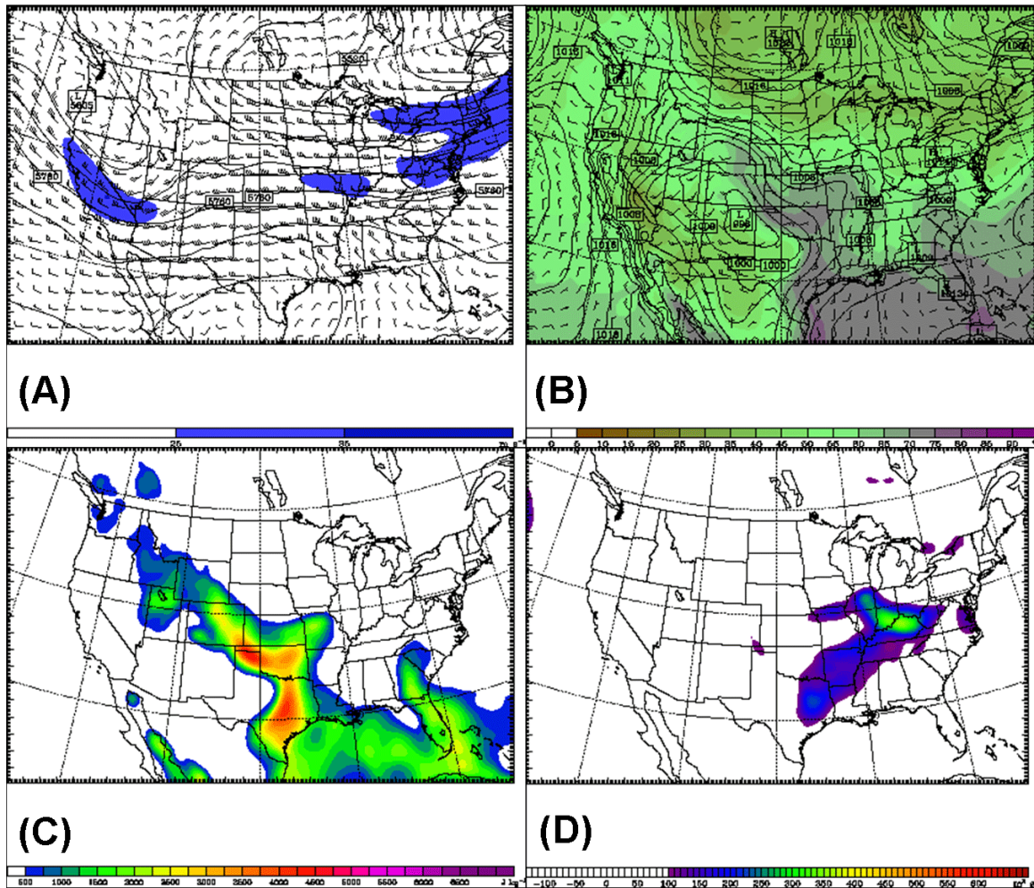
Figure 15: As in Fig. 14, valid at 0000 UTC 3 June 1993. Click image to enlarge.
