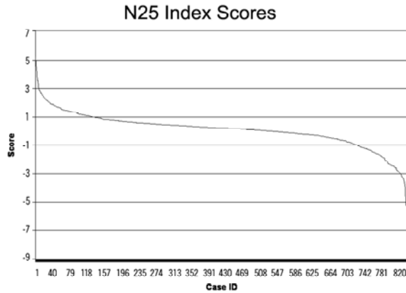
Figure 1: Plot of the values of the N25 index scores for the 840 cases considered in the current study. Click image to enlarge.
