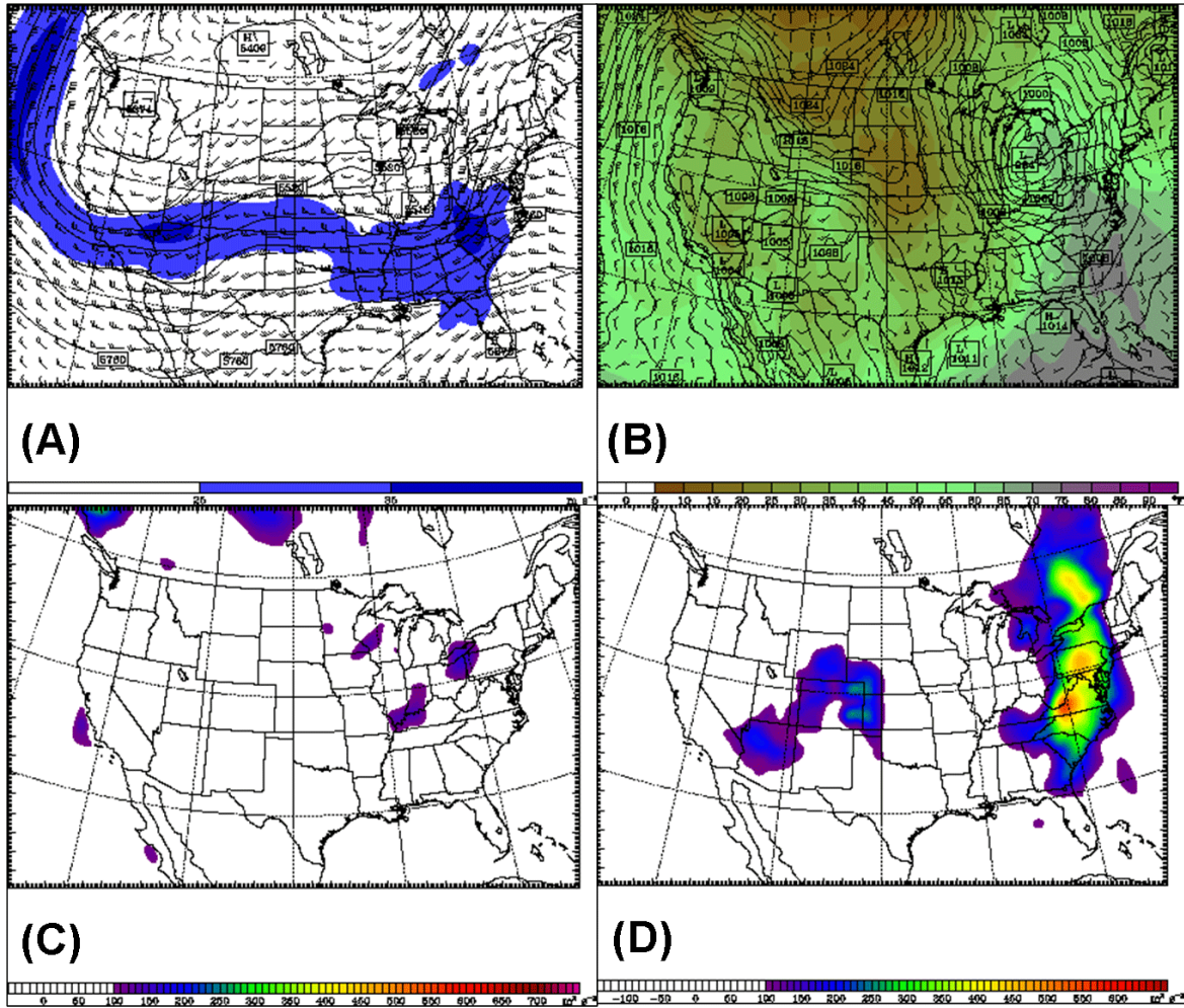
Figure 14: NARR fields valid at 0000 UTC 10 November 2000 of: a) 500-hPa winds (barbs in kt), isotachs (filled contours in \text{m s}^{-1} ), and geopotential heights (contours in m); b) surface dew point temperature (filled contours in ^{\circ}\text{F} ), winds (barbs in kt), and mean sea-level pressure (contours in hPa); c) SBCAPE ( \text{J kg}^{-1} ); and d) 0–1 km SREH ( \text{m}^2 \text{s}^{-2} ). Click image to enlarge.
