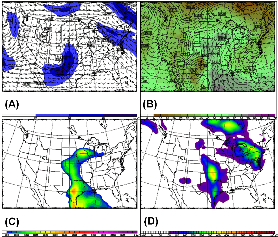
Figure 16: As in Fig. 14, valid at 0000 UTC 8 March 2000. Click image to enlarge.
