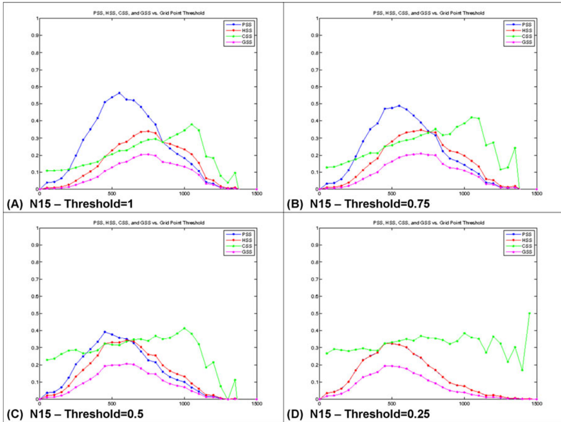
Figure 7: a) Same as Fig. 6d. b), c), d) As in (a), with the N15 index threshold, used to discriminate major from intermediate and marginal outbreak days, changed to 0.75, 0.5 and 0.25 respectively. Click image to enlarge.
