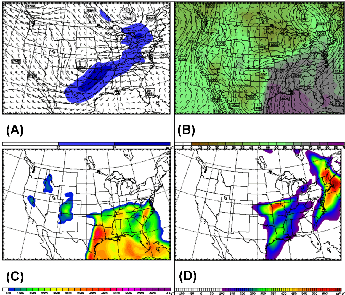
Figure 17: As in Fig. 14, valid at 0000 UTC 18 May 1995. Click image to enlarge.
