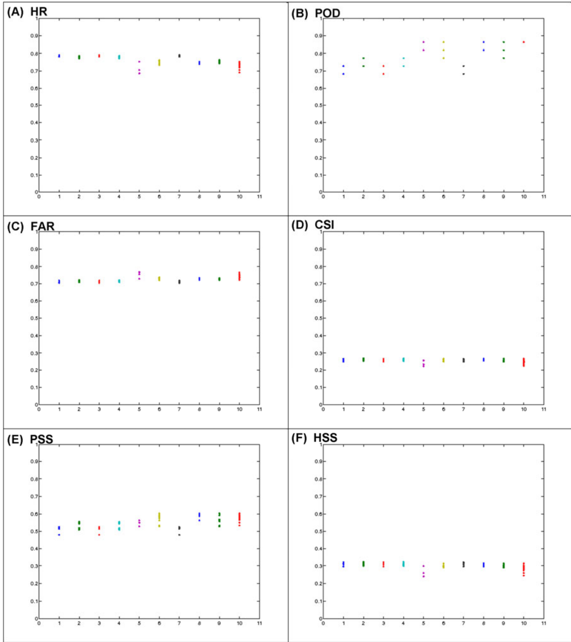
Figure 11: Contingency statistics (labeled) of 25 statistical models developed from the training data, using the mean hypothetical distance a storm travels through the area in which the unconstrained STP \geq 1 as the diagnostic criterion, and the N15 index as the verifying outbreak classification criterion. Statistical algorithm IDs are on the x-axes and are identified in Table 1. Statistical models with the same contingency scores as others are overlain on preceding dots. Click image to enlarge.
