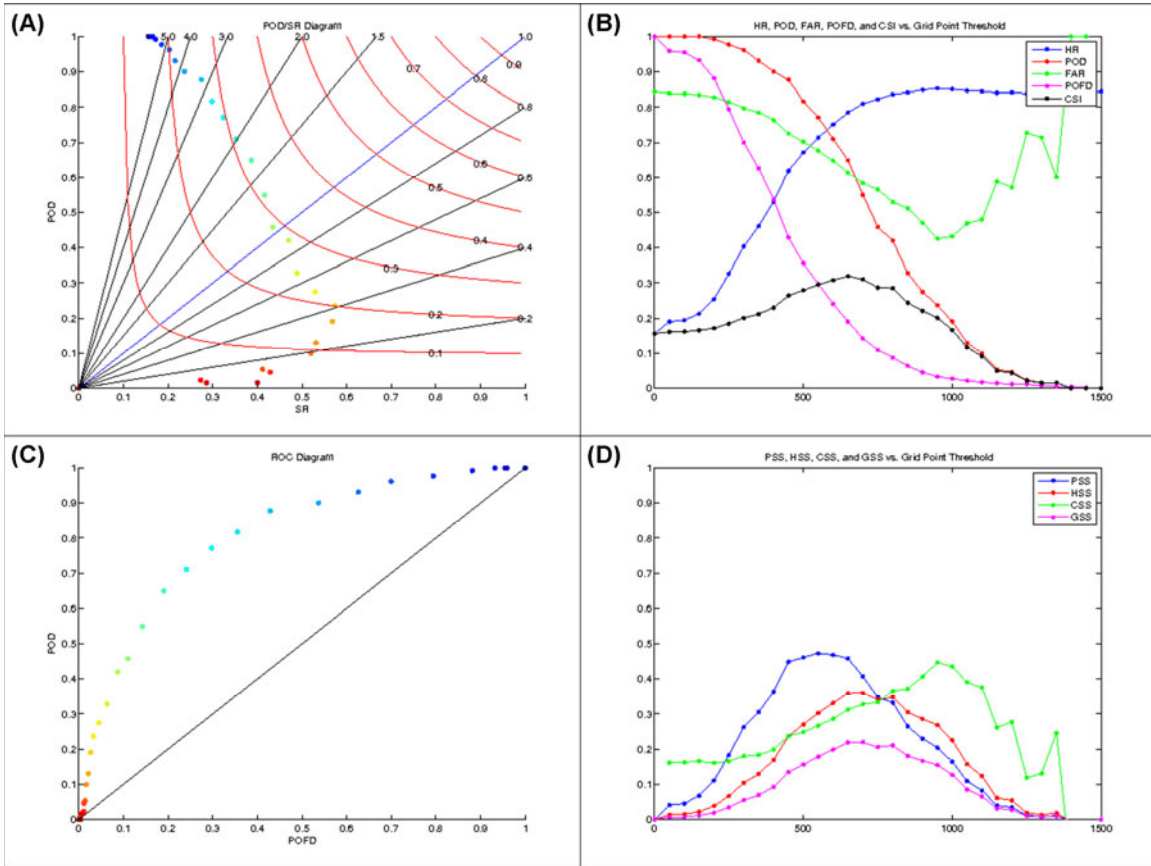
Figure 5: As in Fig. 4, using the mean hypothetical storm distance in the area through which the unconstrained STP \geq 1 . Click image to enlarge.
