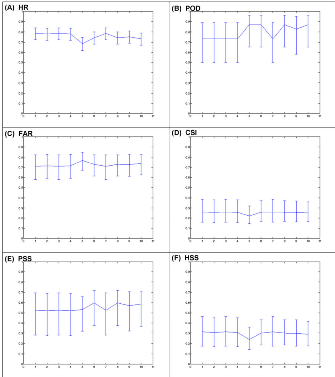
Figure 12: Bootstrap 95% confidence intervals of the contingency statistics (labeled) for the testing set, using all 630 training cases. The medians are shown by the connecting line for each of the 10 statistical models ( x -axes; algorithms identified in Table 1). Threshold and outbreak classification criteria as in Fig. 11. Click image to enlarge.
