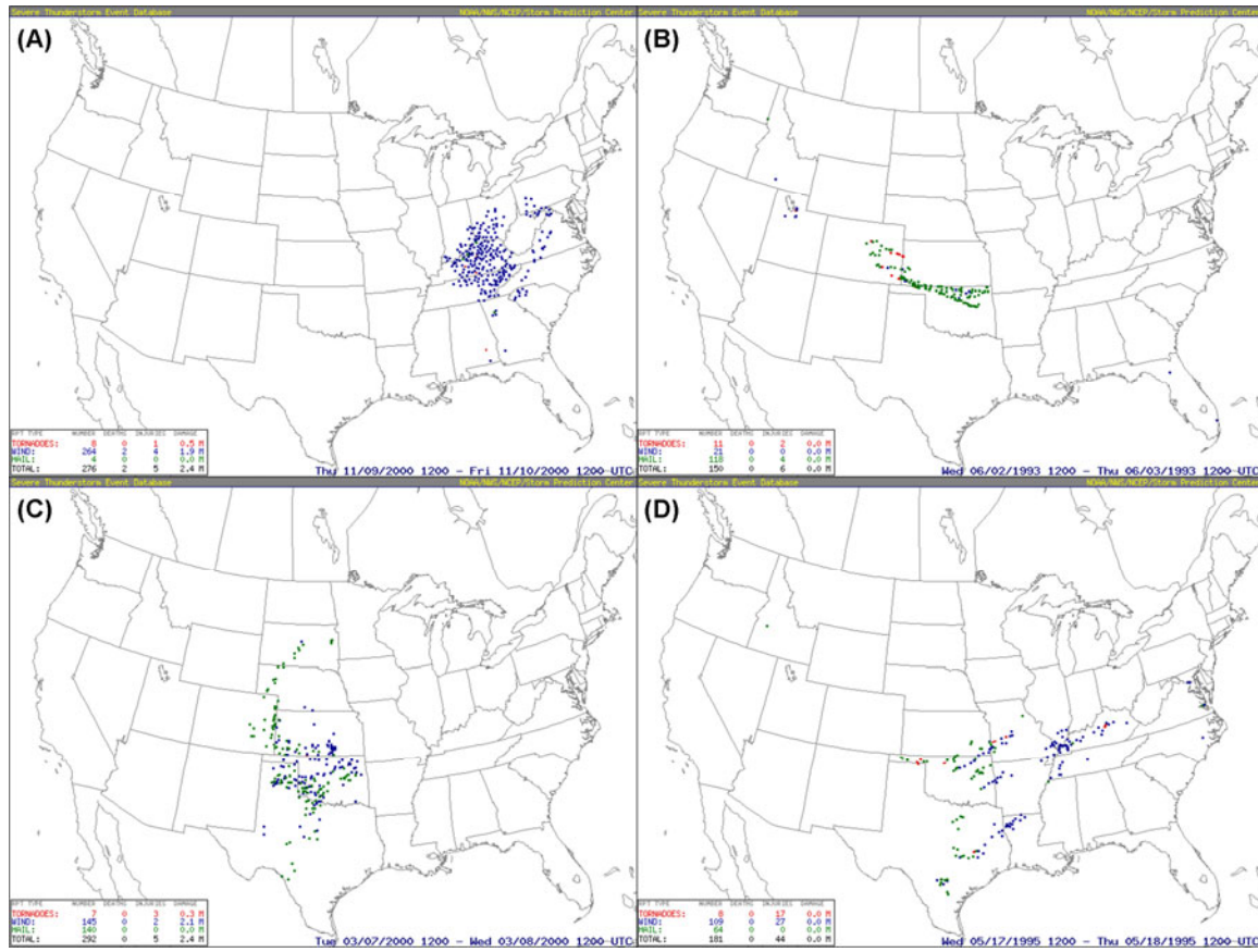
Figure 13: Severe reports from 1200 UTC on the indicated date to 1200 UTC the following day, with red dots denoting tornadoes, green dots denoting large hail, and blue dots denoting wind gusts or wind damage, for the a) 9 November 2000, b) 2 June 1993, c) 7 March 2000, and d) 17 May 1995 outbreak days. Click image to enlarge.
