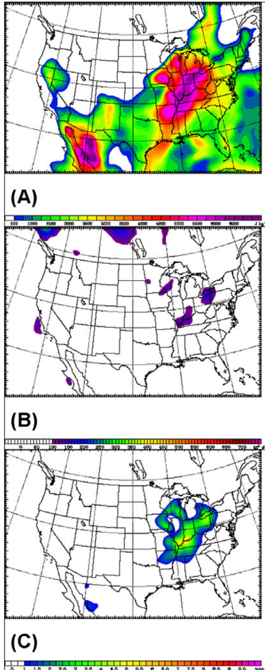
Figure 3: NARR fields of a) SBCAPE ( \text{J kg}^{-1} ), b) 0–1 km AGL SREH ( \text{m}^2 \text{s}^{-2} ), and c) 0–1 km AGL EHI, valid at 0000 UTC 30 August 1984. Click image to enlarge.
